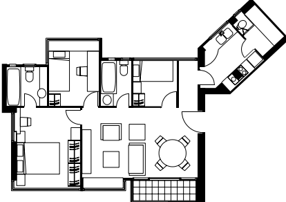
Apartment 25A 3-bedroom + maid room
